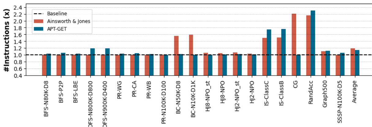
Figure 11. The overhead of injected prefetching instructions over non-prefetching baseline: APT-GET increases the total number of instructions 1.14× in average, compared to 1.19× in average of Ainsworth & Jones, over non-prefetching baseline.
